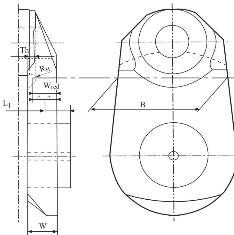
Crankshaft without overlap
