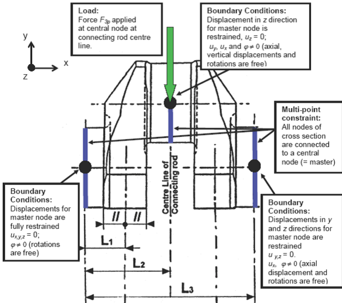
Fig. C.4. Boundary and load conditions for the 3-point bending load case of an inline engine.
