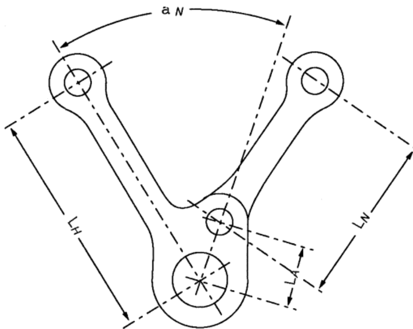
Fig. 1.2 Articulated-type connecting-rod
