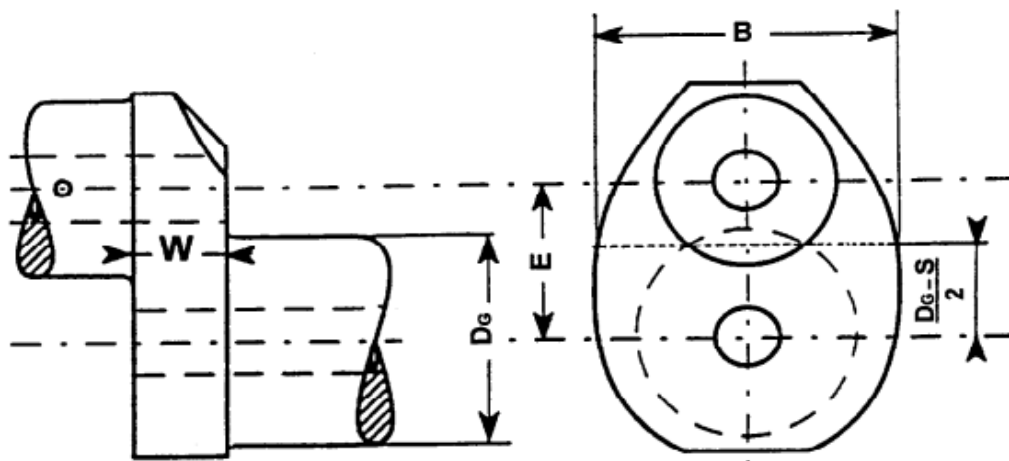
Overlapped crankshaft
