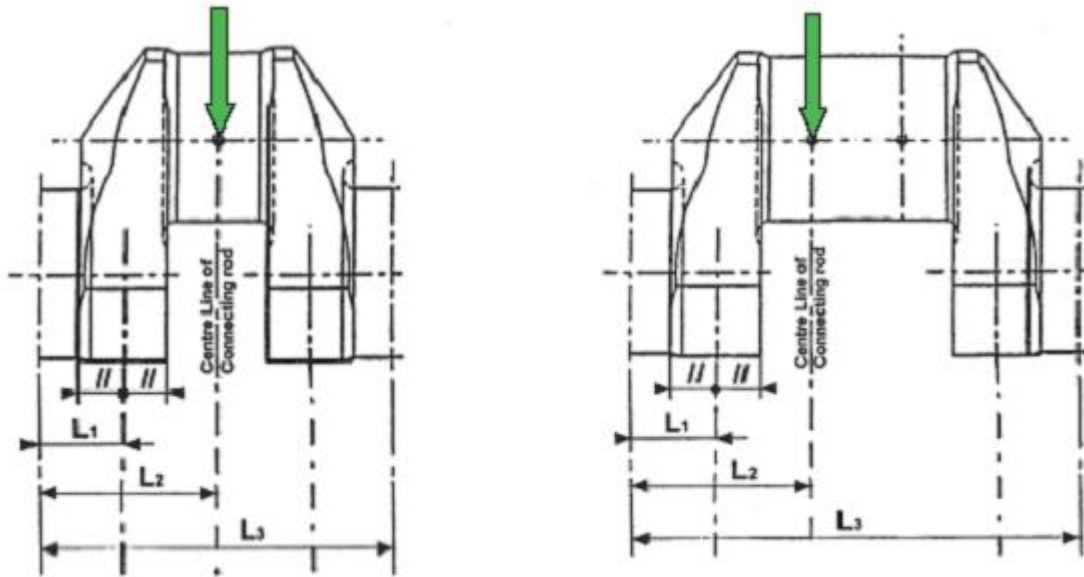
Fig. C.5 Load applications for in-line and V-type engines.
