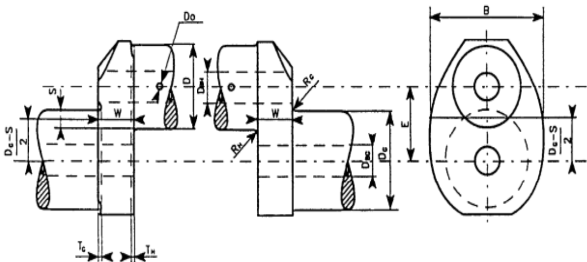
Fig. 2.5 Crank dimensions
