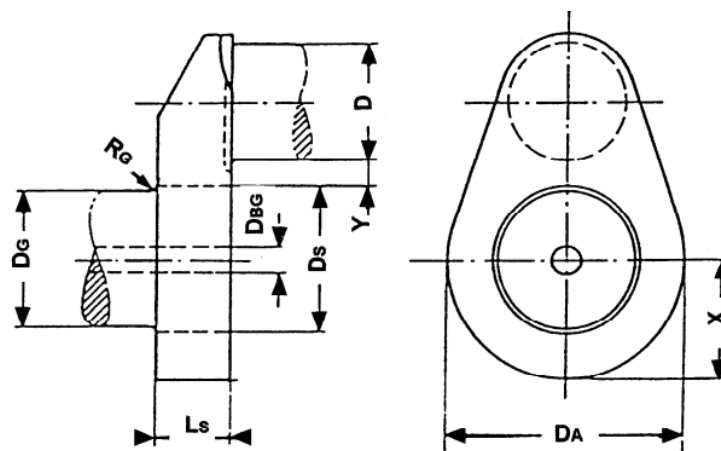
Fig. 2.6 Crankthrow of semi-built crankshaft
