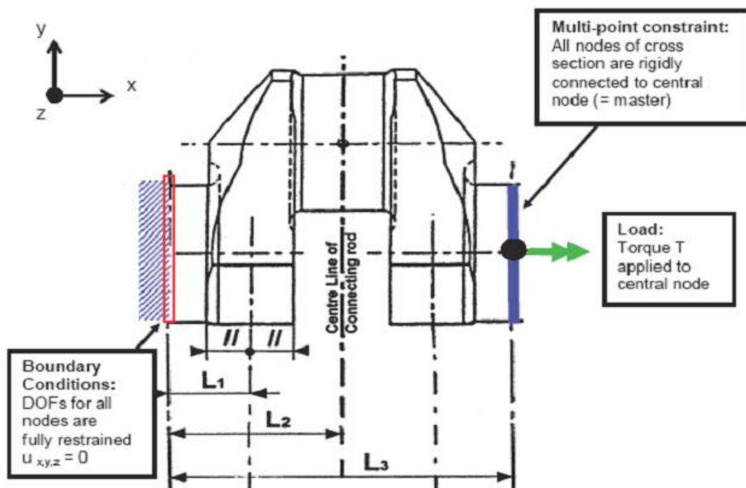
Fig. C.2 Boundary and load conditions for the torsion load case.
