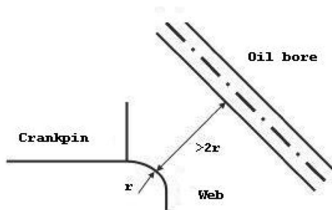
Fig. C.1. Oil bore proximity to fillet.
