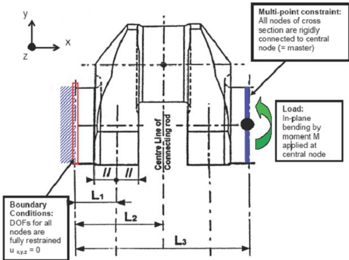
Fig. C.3 Boundary and load conditions for the pure bending load case.
