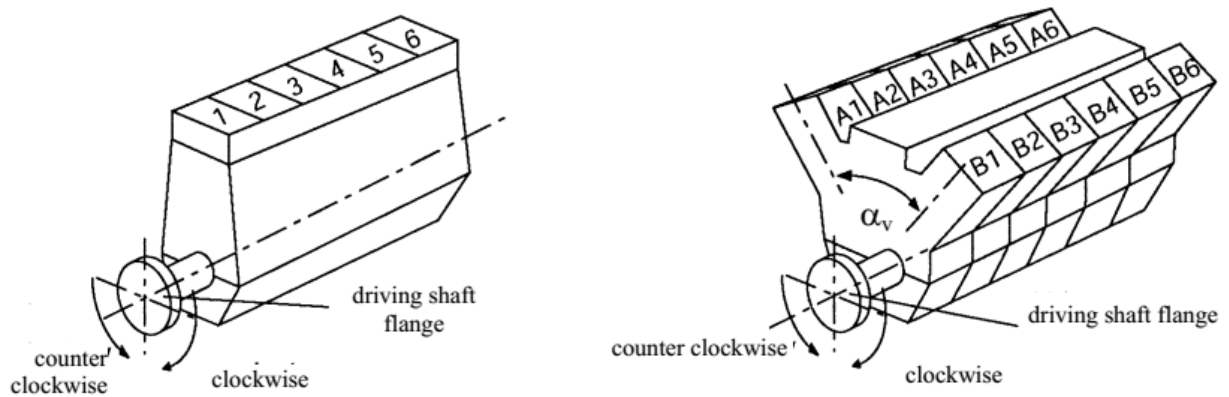
Fig. 1.1 Designation of the cylinders
