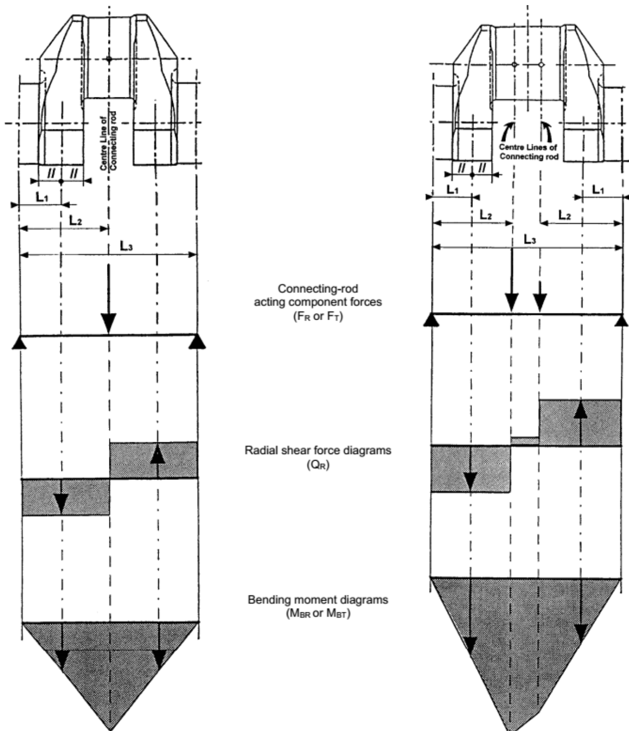
Fig. 2.1 Crankthrow for in line engine
