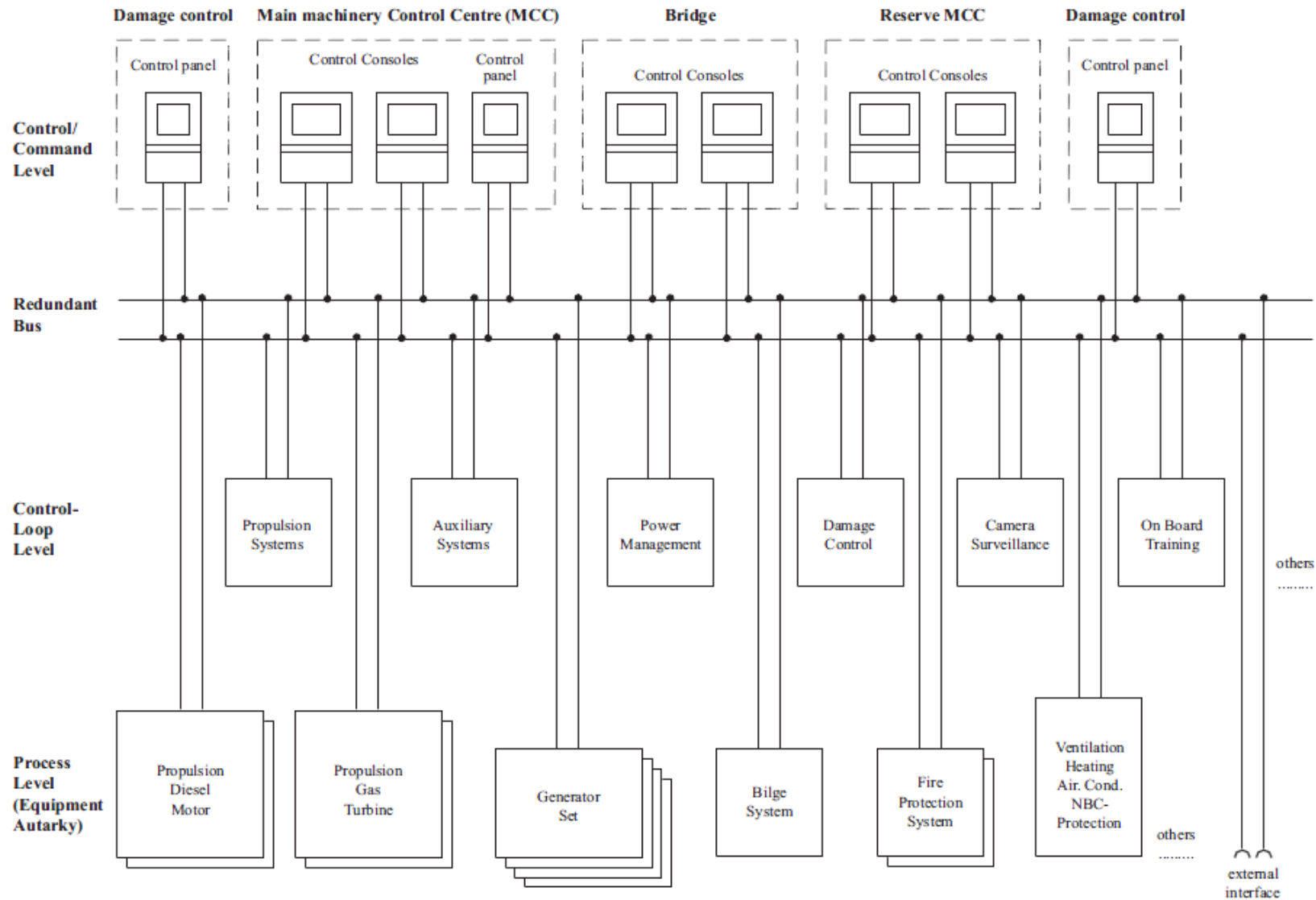
Fig.7.1 Hierarchical structure of integrated system (example)
