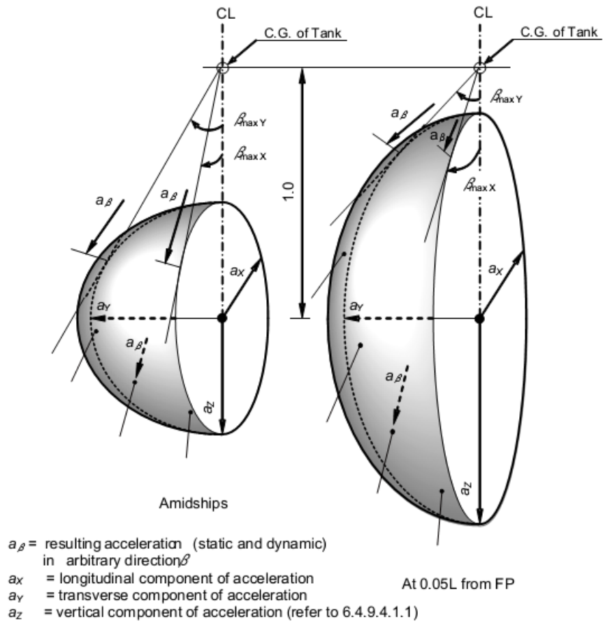
Figure 6.4.1: Acceleration Ellipsoid
