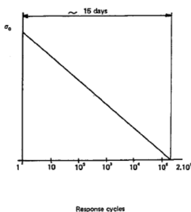
\sigma_0 = most probable maximum stress over the life of the ship Response cycle scale is logarithmic; the value of 2.10^6 is given as an example of estimate.
