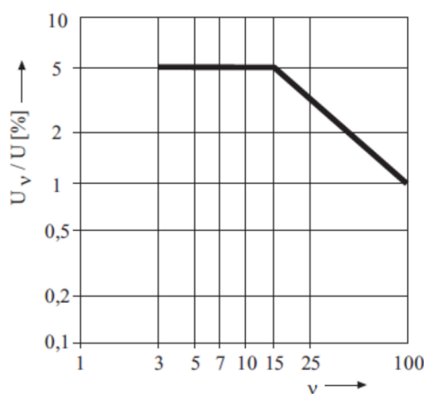
Figure 1.1: Limit values for the single harmonics in the supply voltage. U_v is the RMS value of the v -th order harmonic voltage
