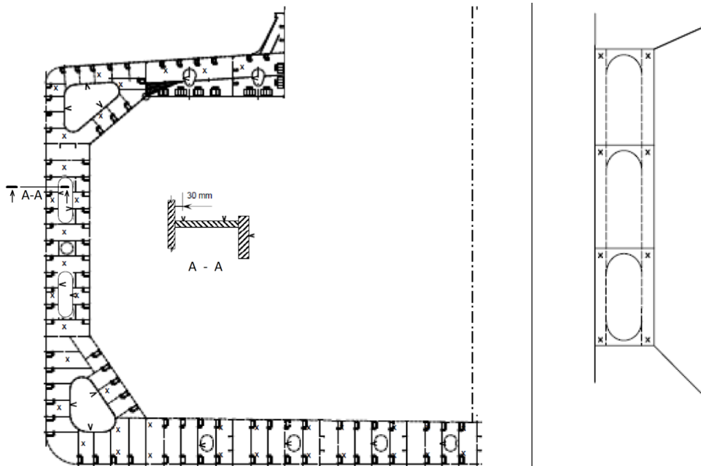
Double skin bulk carrier
