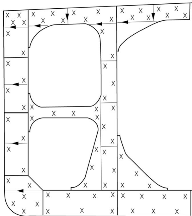
Figure 1.13: Transverse rings in cargo and ballast tanks
