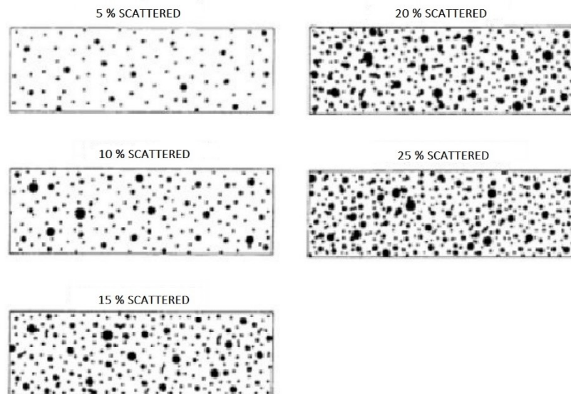
Figure 1.1: Pitting intensity diagrams
