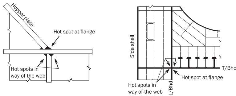
Figure 17 : Web-stiffened cruciform joints
