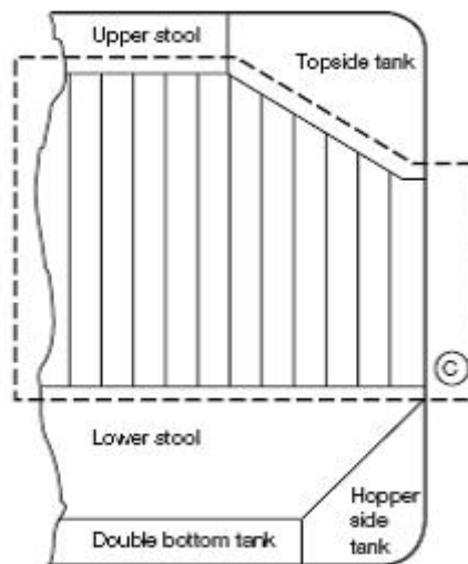
Figure 1.10: Close-up Survey and Thickness Measurement Areas for double skin Bulk carrier
