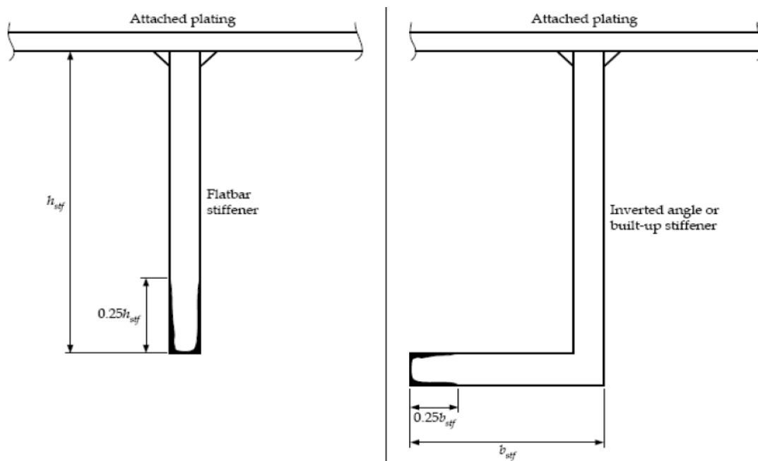
Figure 1.2: Edge corrosion
