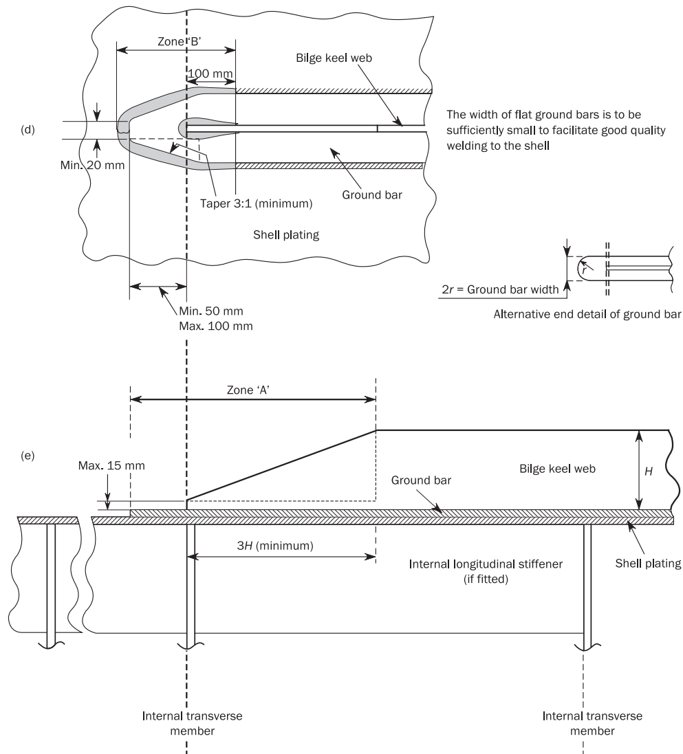
Figure 20 : Bilge keel end design (continued)
