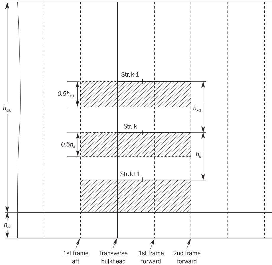
Figure 8 : Region for stringer correction, t_r , for ships with 3 stringers
