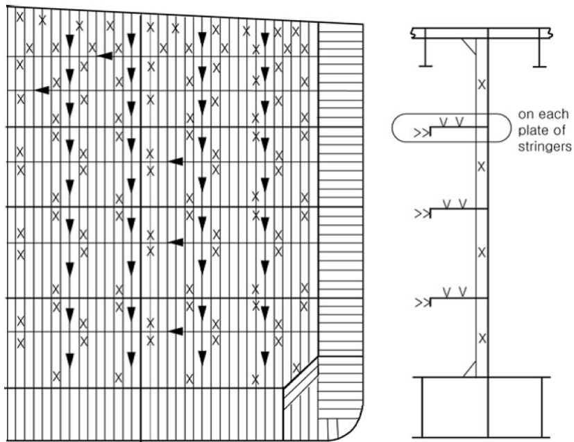
Figure 1.14: Transverse bulkheads in cargo tanks
