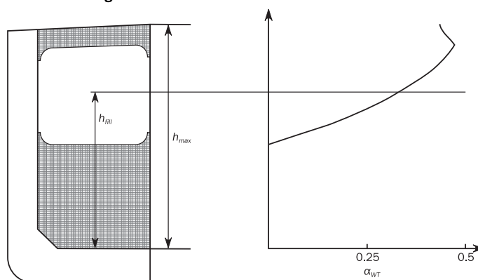
Figure 11 : Transverse wash bulkhead coefficient
