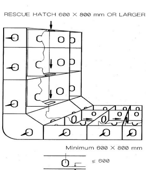
Figure 3.5(a) Access through side ballast space and double bottom
