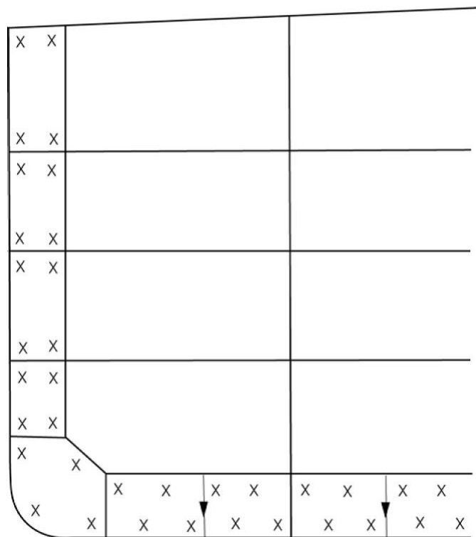
Figure 1.15: Transverse bulkheads in ballast tanks
