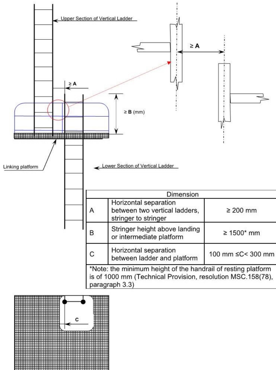
Figure 3.3: Vertical Ladder - Ladder through the linking platform
