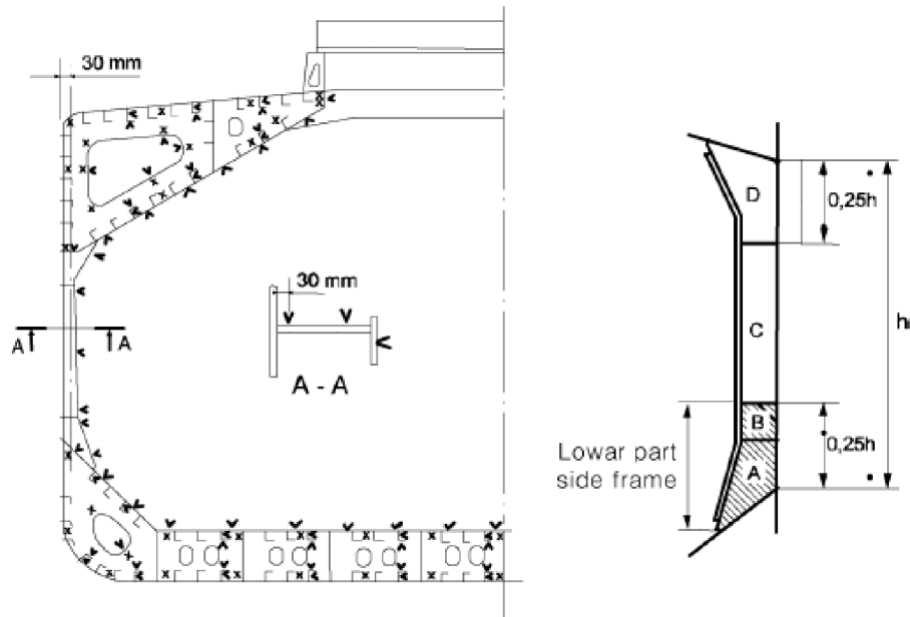
Single skin bulk carrier
