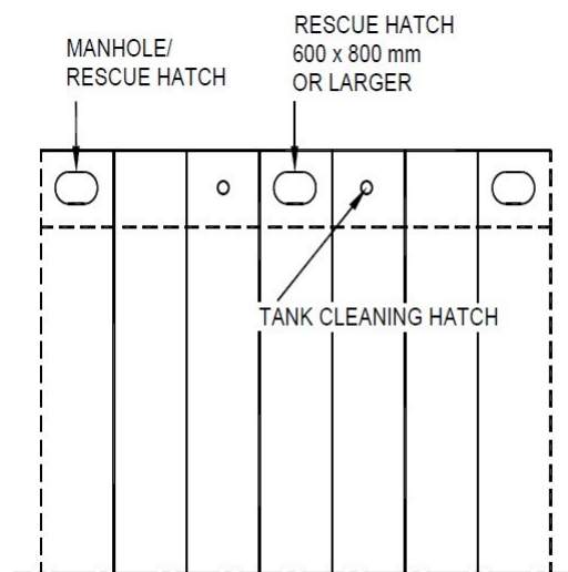
Figure 3.5(b) Access through deck into wing ballast space
