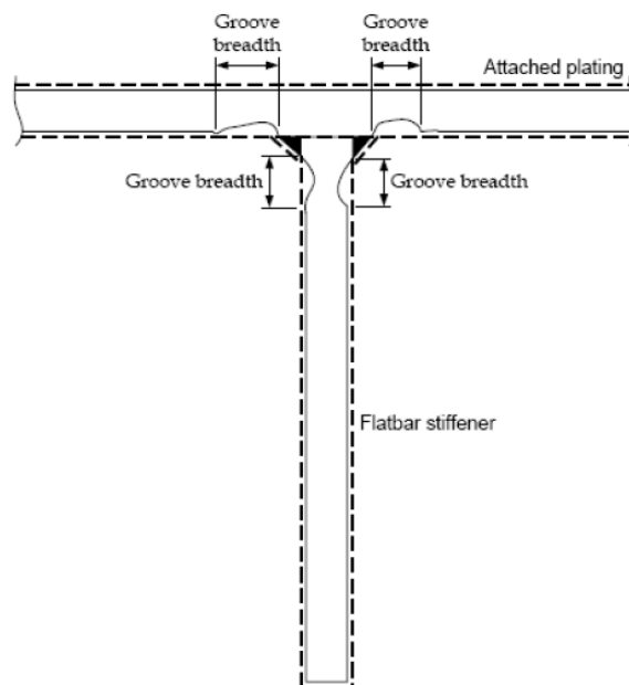
Figure 1.3: Grooving corrosion
