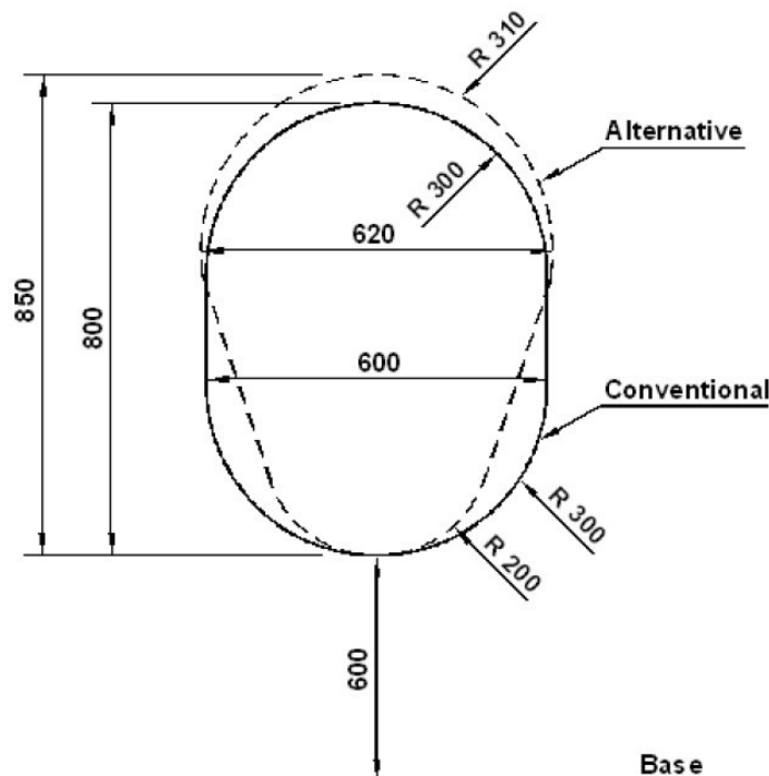
Figure 3.2: Access opening in vertical structure
