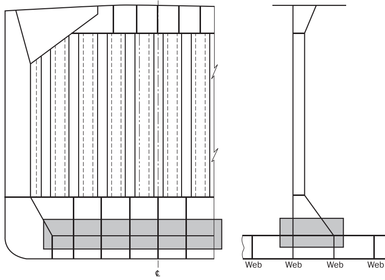
Figure 5 : Screening areas at connections of lower stool to inner bottom and hopper tank
