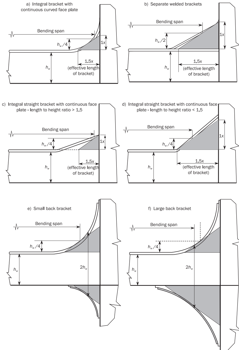
Figure 9 : Effective bending span of primary supporting member
