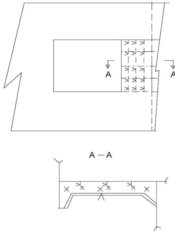
Figure 1.9: Locations of measurements on underdeck structure
