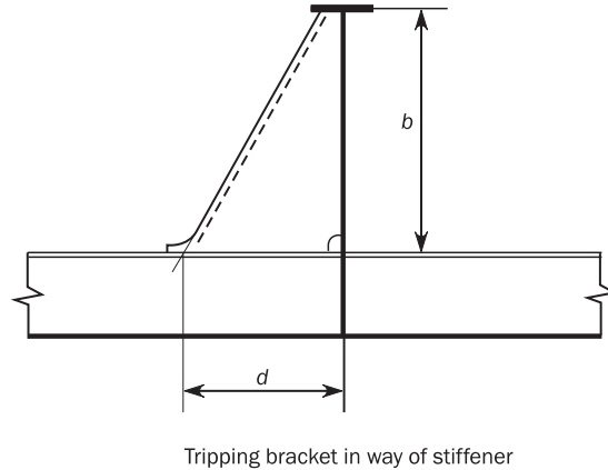
Figure 4 : Primary supporting member: Tripping bracket arrangement
