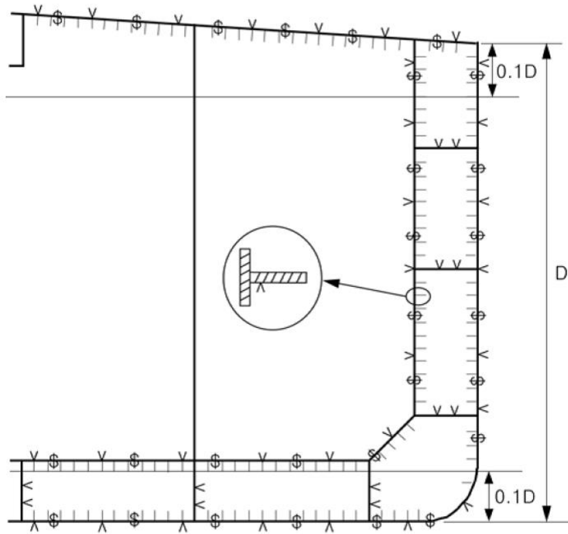
Figure 1.12: Transverse section
