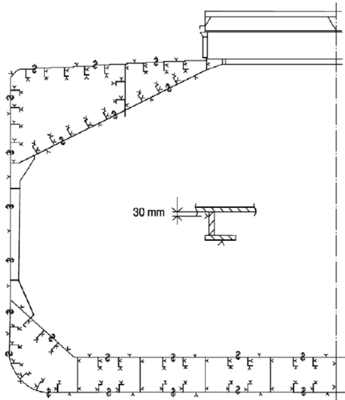
Single skin Bulk Carrier
