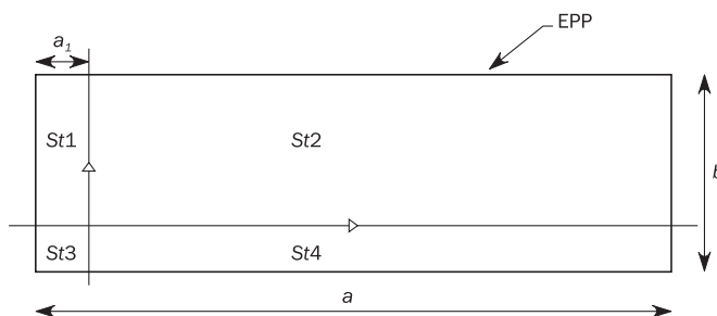
Figure 17 : Strake considered in a given EPP
