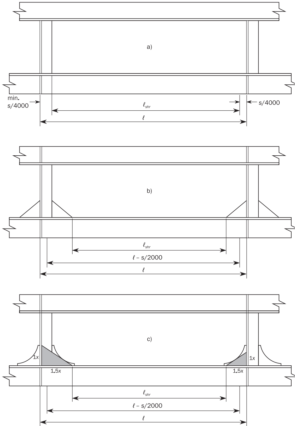
Figure 6 : Effective shear span for local support members with continuous face plate along bracket edge
