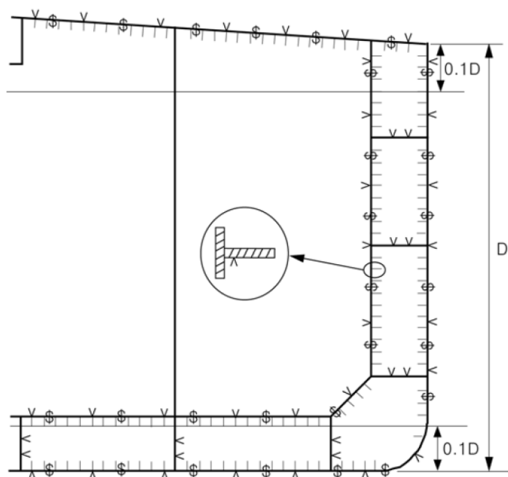
Fig. 1.12 Transverse section
