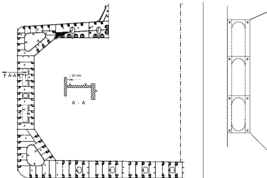
Double skin bulk carriers
