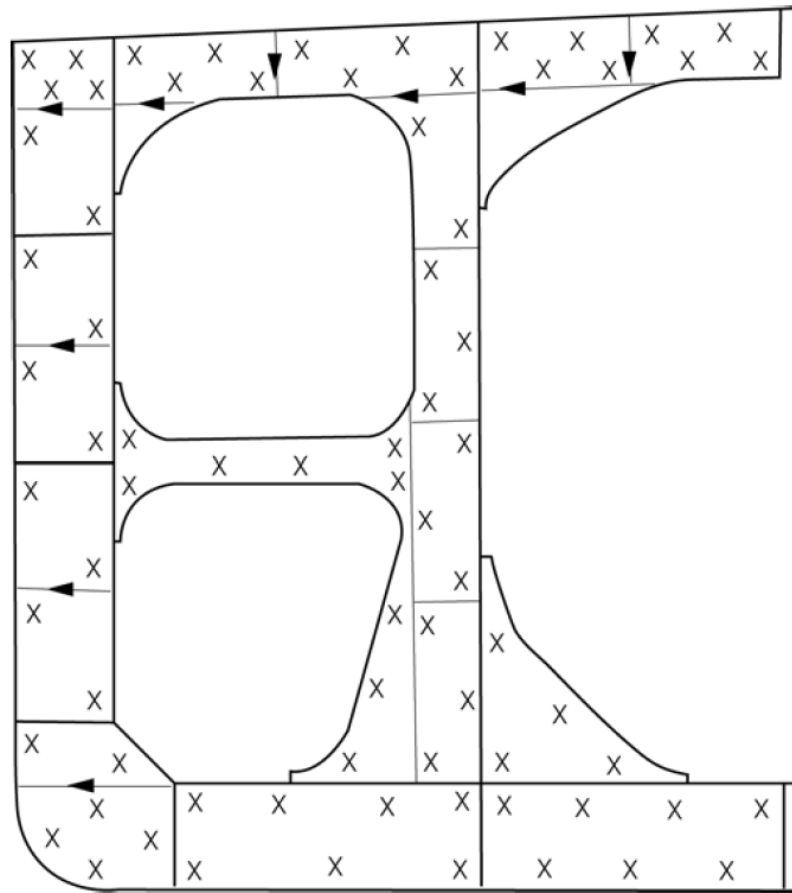
Fig. 1.13 Transverse rings in cargo and ballast tanks
