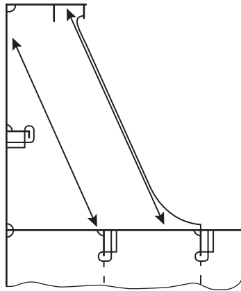
Figure 6 : Coaming stay (example 1)
