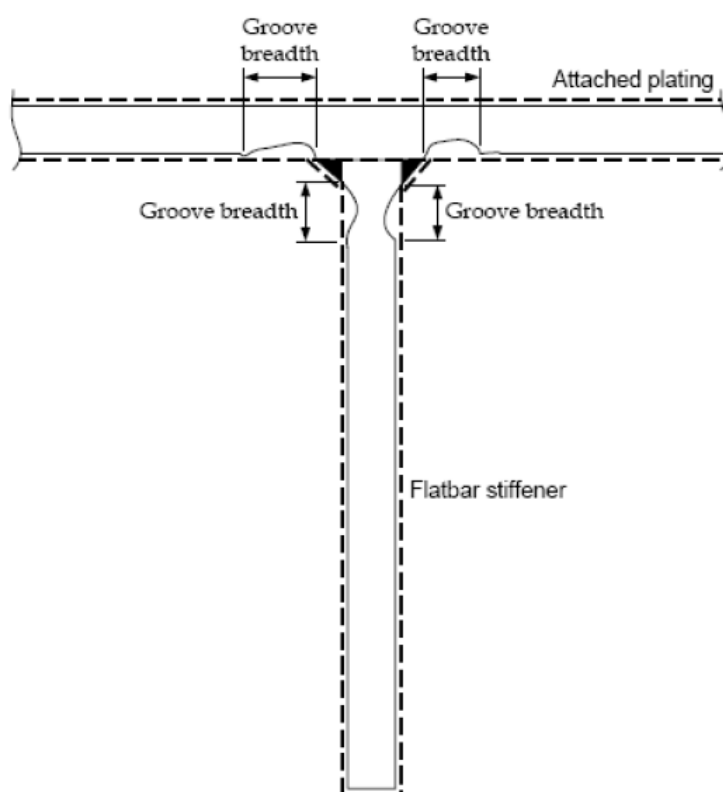
Fig. 1.3 Grooving corrosion
