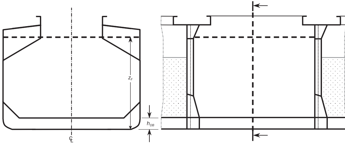
Figure 7 : Flooded cargo hold without cargo
