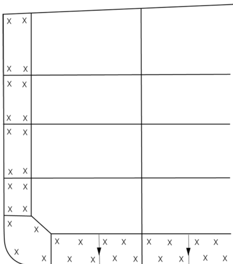
Fig. 1.14 Transverse bulkheads in ballast tanks
