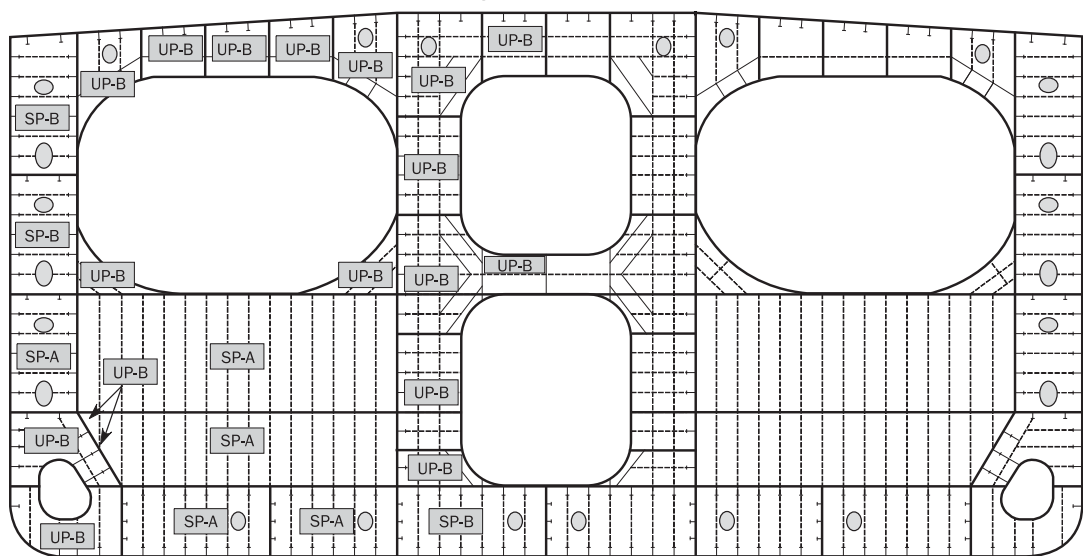
Figure 4 : Cross tie
