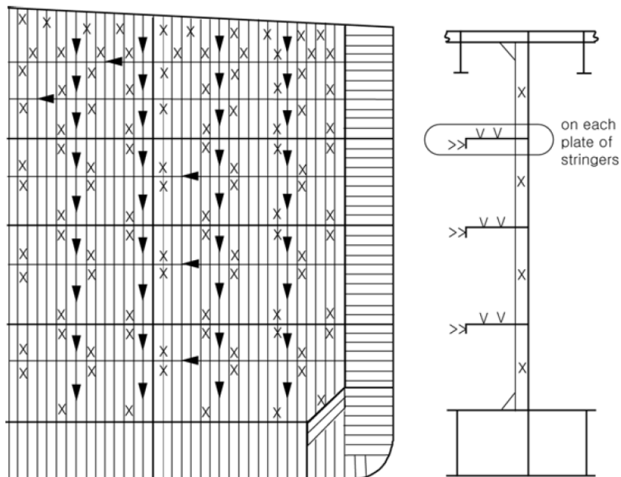
Fig. 1.14 Transverse bulkheads in cargo tanks
