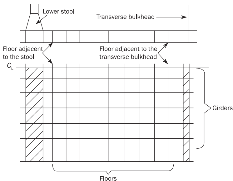
Figure 7 : Double bottom structure
