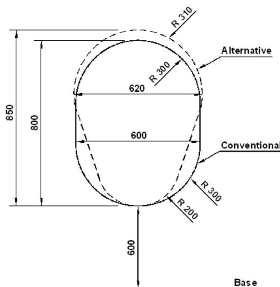
Fig. 3.2 Access opening in vertical structure
