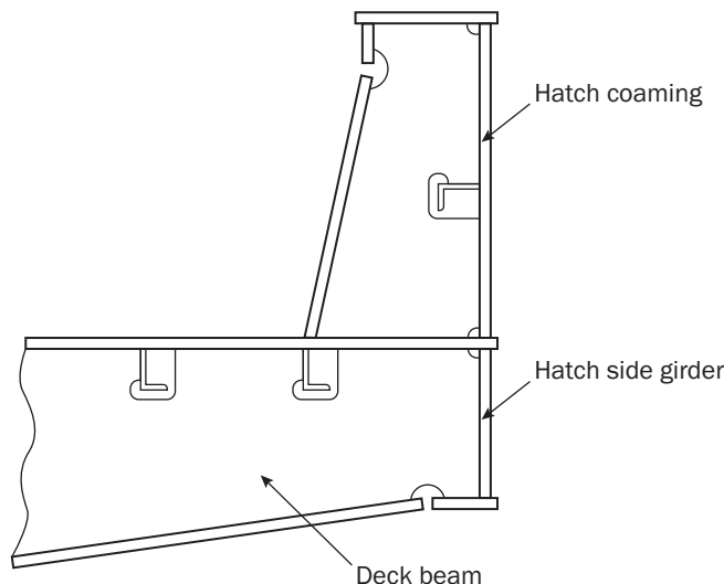
Figure 1 : Example of extension to lower edge of deck beams of longitudinal coaming by fitting a hatch side girder [CORR1 to 01 JAN 2021]
