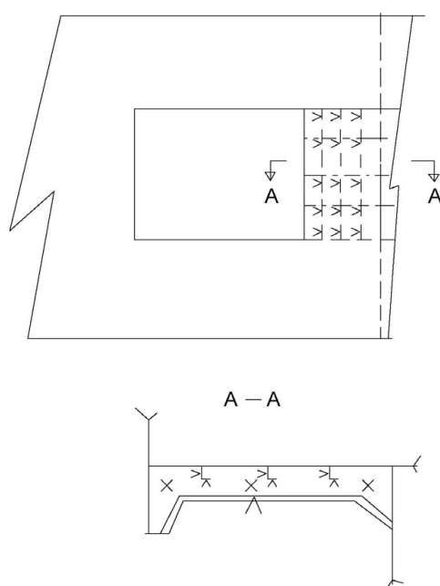
Fig. 1.9 Locations of measurements on underdeck structure
