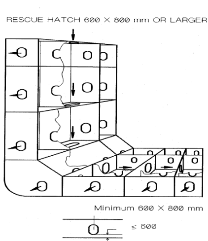
Fig.3.5(a) Access through side ballast space and double bottom
