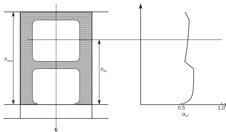
Figure 12 : Transverse web frame coefficient
