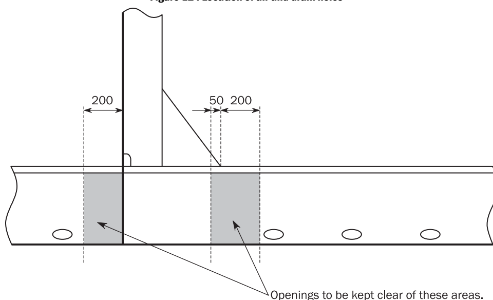
Figure 12 : Location of air and drain holes
