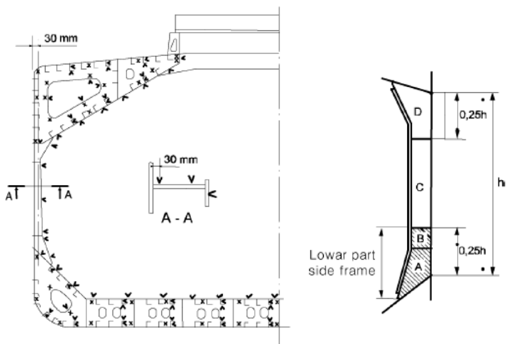
Single skin bulk carriers
