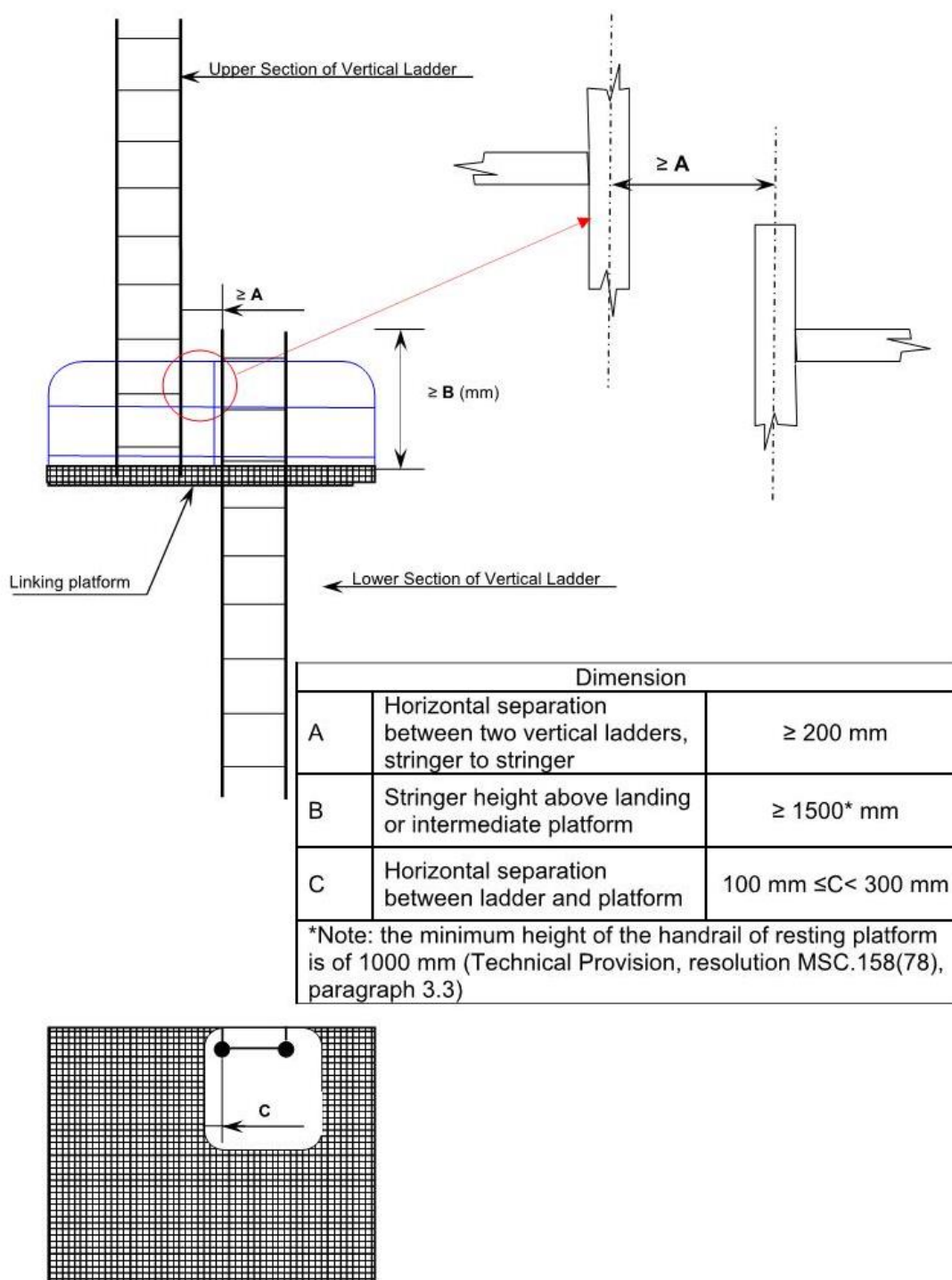
Fig. 3.3 Vertical Ladder – Ladder through the linking platform
