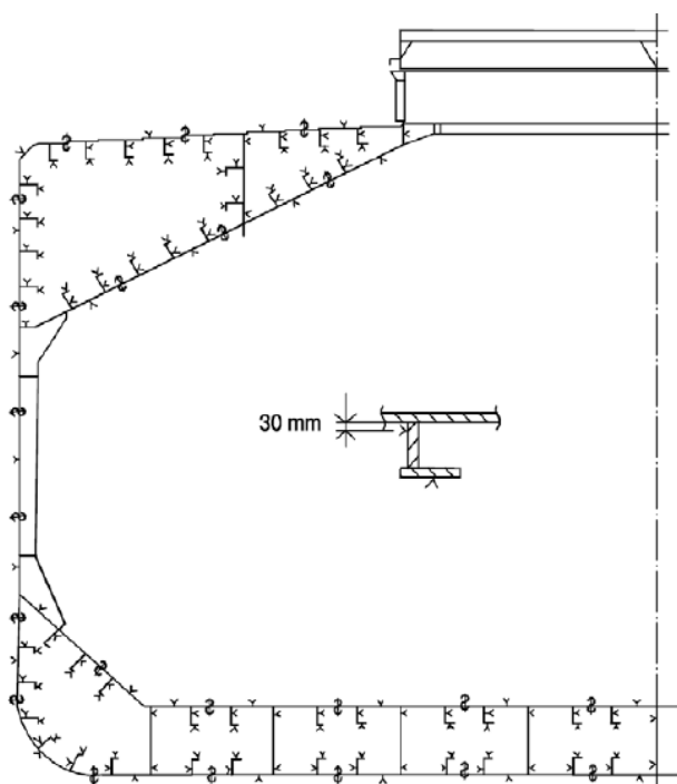
Single skin Bulk Carrier
