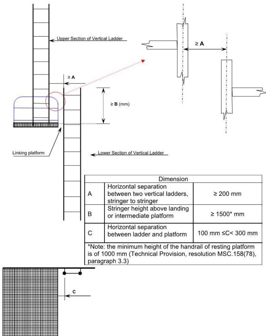
Fig. 3.4 Vertical Ladder – Side Mount
