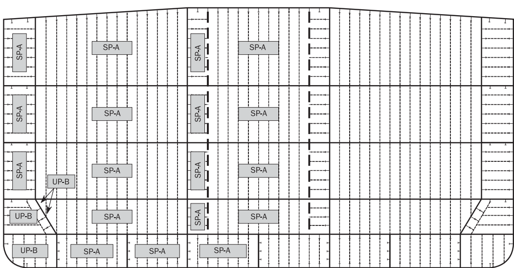
Figure 3 : Transverse bulkhead for oil tankers
